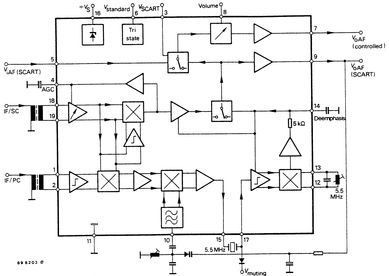
Figure 1 Block diagram
